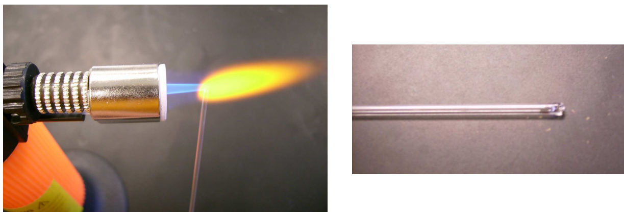
Figure 1. Flame Sealing the Capillary Internal Standard with a Micro-torch.
