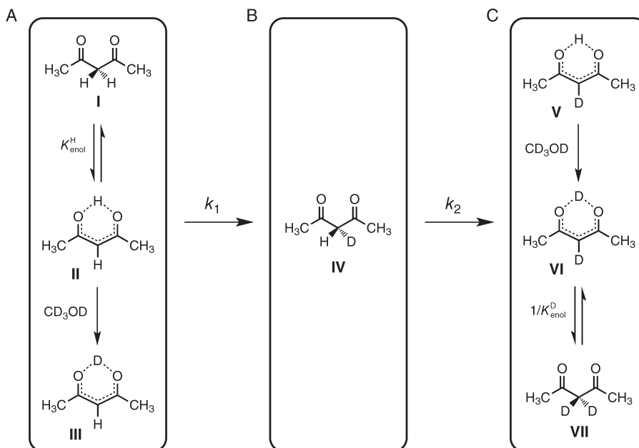
Scheme 2. A Detailed Reaction Scheme for the Deuterium Exchange between Acetylacetone and CD 3 OD a
