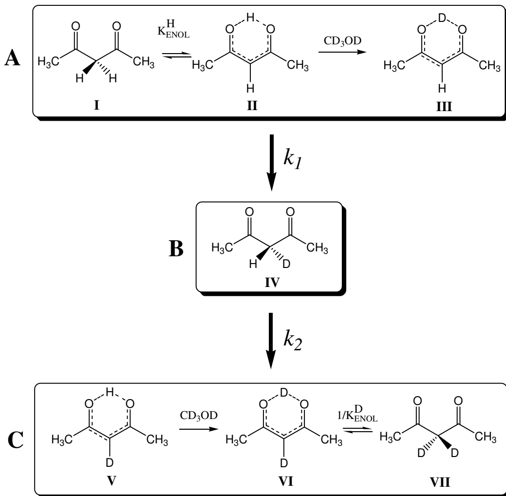
Figure 5. A Simplified Reaction Scheme for the Deuterium Exchange Between Acetylacetone and \text{CD}_3\text{OD} .
