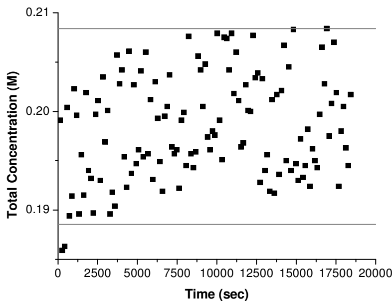
Figure 4. Variation in the Total (Ketone + Enol) Concentrations for (a) Acetylacetone and (b) Ethyl Acetoacetate During the Course of a Kinetic Experiment. The horizontal lines represent \pm 5\% variation around the average concentration.
