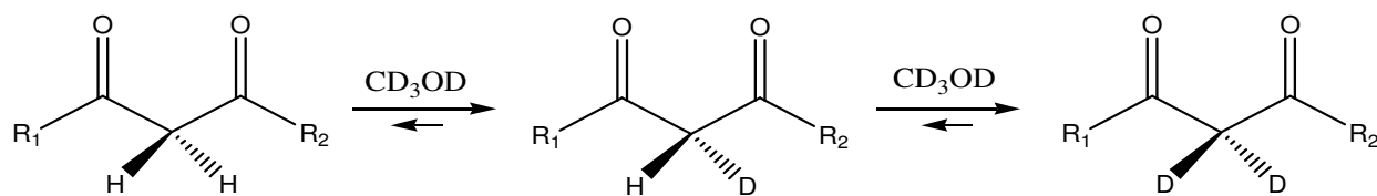
Figure 3. Deuterium Exchange Reactions Between \text{CD}_3\text{OD} and a \beta -Dicarbonyl Compound.
