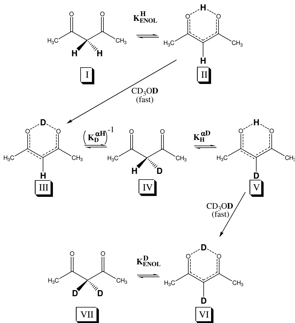
Figure 4. A Proposed Mechanism of Deuterium Exchange Between \text{CD}_3\text{OD} and Acetylacetone.
