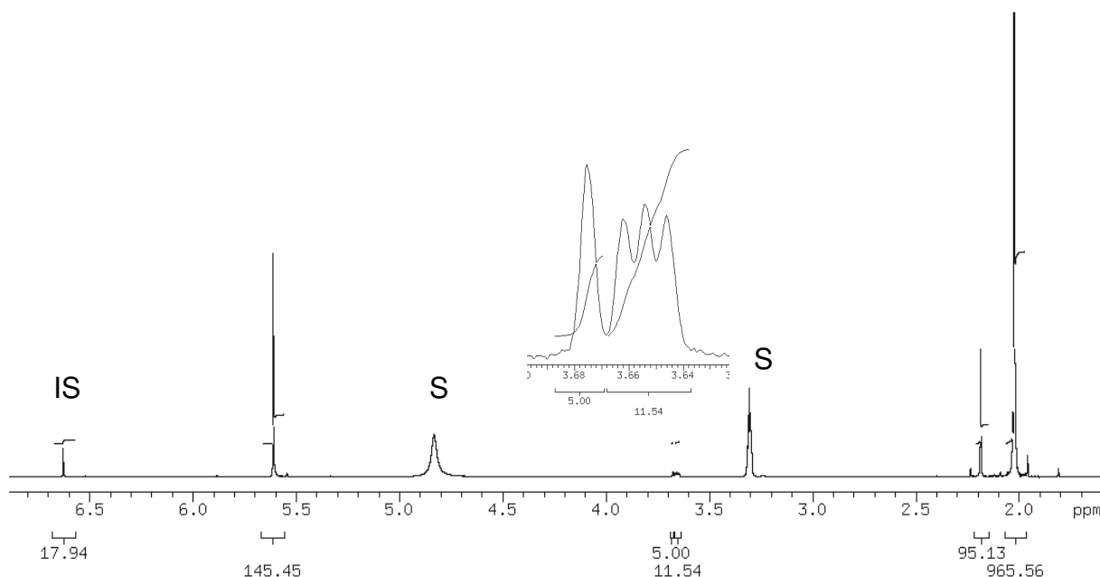
Figure 6. An Example NMR Spectrum from the Reaction of Acetylacetone and \text{CD}_3\text{OD} at 25^\circ\text{C} . The reaction time was 8 minutes. The inset shows the singlet and 1:1:1 triplet of species I and IV , respectively. The resonances corresponding to the benzene internal standard (IS) and of the \text{CD}_3\text{OD} solvent (S) are indicated.
