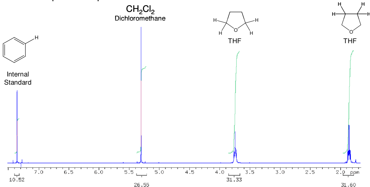
Figure 2. Sample Internal Standard Calibration NMR Spectrum.
