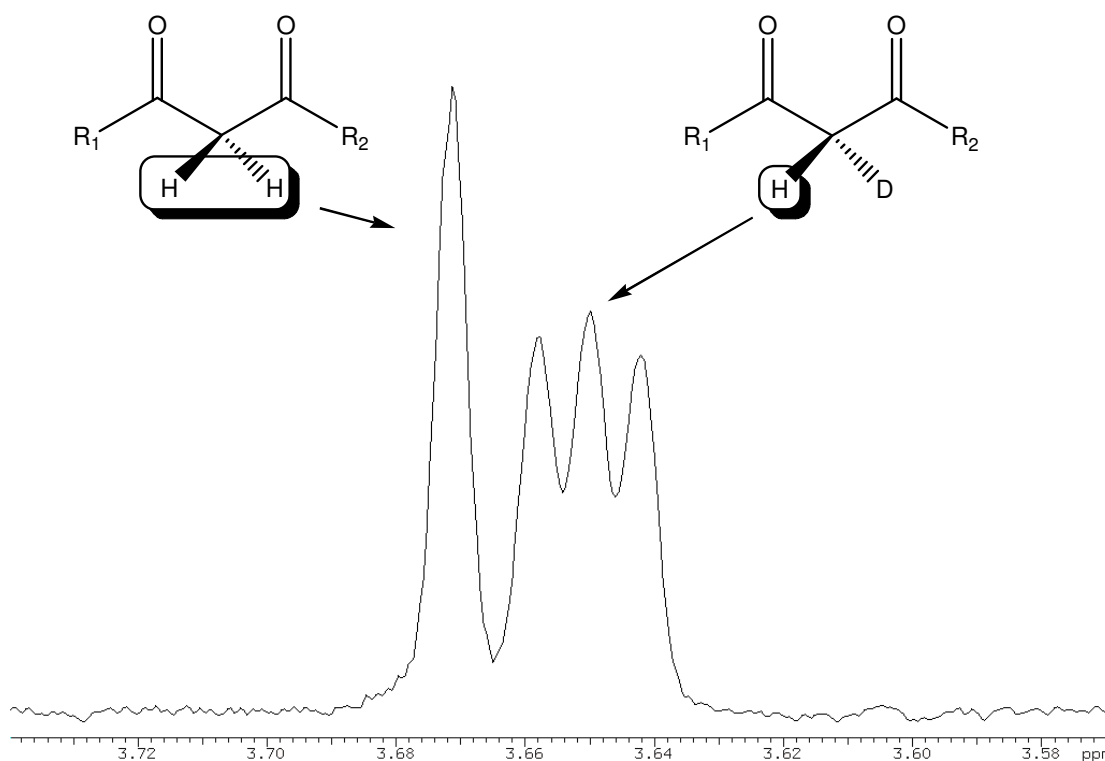
Figure 2. The Effect of Deuterium Substitution on the 1 H-NMR Spectrum of the α-Methylene Position of β-Diketones or β-Ketoesters.
