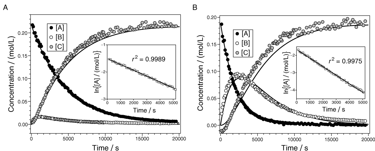
Figure 1. Kinetic modeling of the deuterium exchange reaction as a first-order consecutive process for (A) acetylacetone and (B) ethyl acetoacetate.
