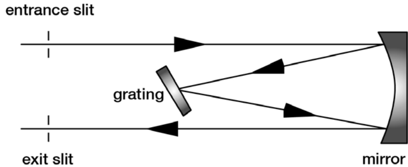
Figure 6-2. The Ebert mount. A single concave mirror replaces the two concave mirrors found in Czerny-Turner mounts.
