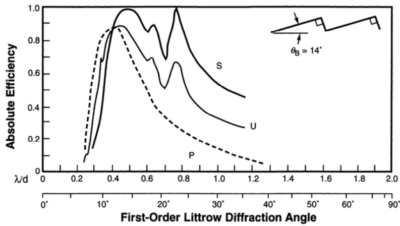
Figure 9-7. Same as Figure 9-5, except 14° blaze angle. The curve for unpolarized light (marked U) is also shown; it lies exactly halfway between the S and P curves.
