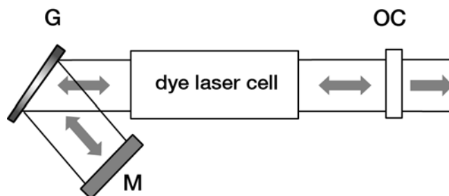
Figure 13-5. The Littman-Metcalf arrangement. The light diffracted by grating G is retroreflected by mirror M, which diffracts the light again back into the dye laser cell.
