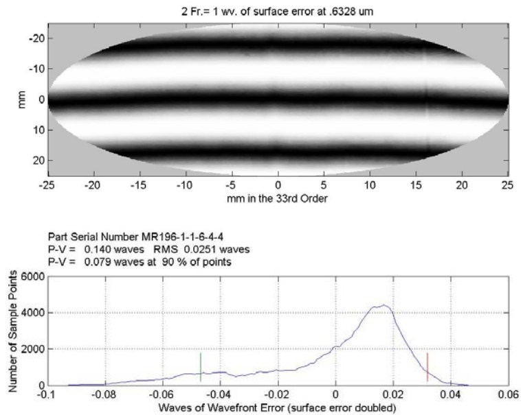
Figure 11-6. Example of an interferogram and histogram generated by a Phase Measuring Interferometer (PMI). In this example, a grating is illuminated in a circular region 50 mm in diameter, and its diffracted wavefront at \lambda = 632.8 nm in the m = 33 order is recorded.
