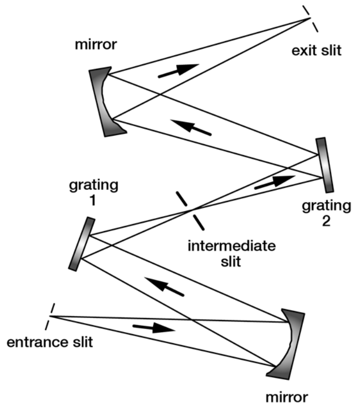
Figure 6-5. A double monochromator mount.
