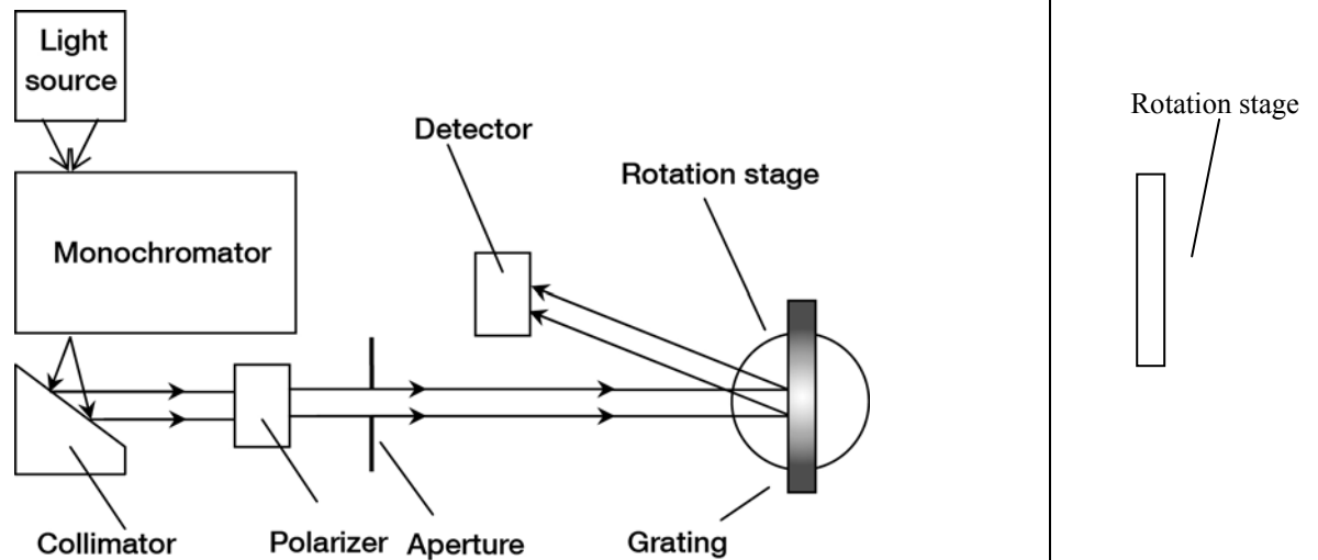
Figure A-1. Typical monochromator-mode efficiency measuring apparatus.
