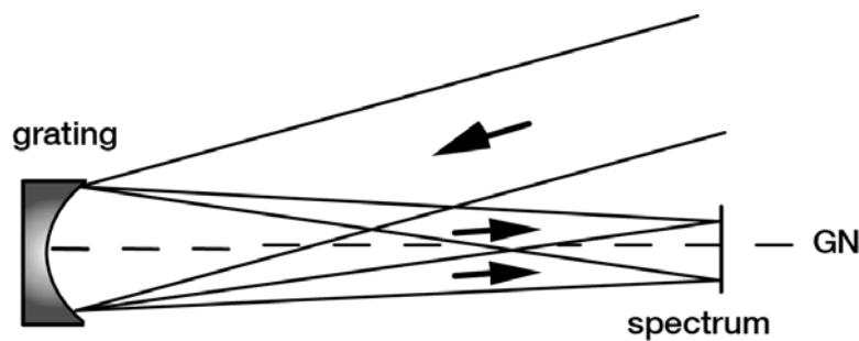
Figure 7-6. The Wadsworth spectrograph. Collimated light is incident on a concave grating; light of two wavelengths is shown focused at different points. GN is the grating normal.
