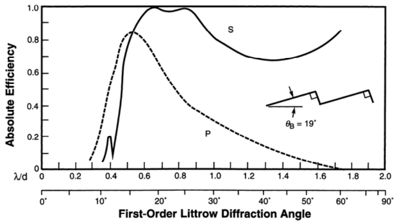
Figure 9-8. Same as Figure 9-5, except 19° blaze angle.
